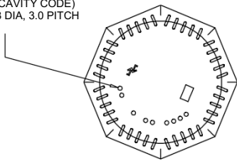
VIEW ON BASE SHOWING EMBOSSED MARKING STANDING AREA EMBOSSED WITH BAR STIPPLE
